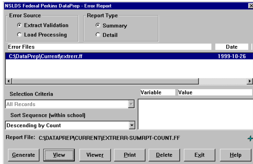
Figure 5-51: Error Report Dialog Box
