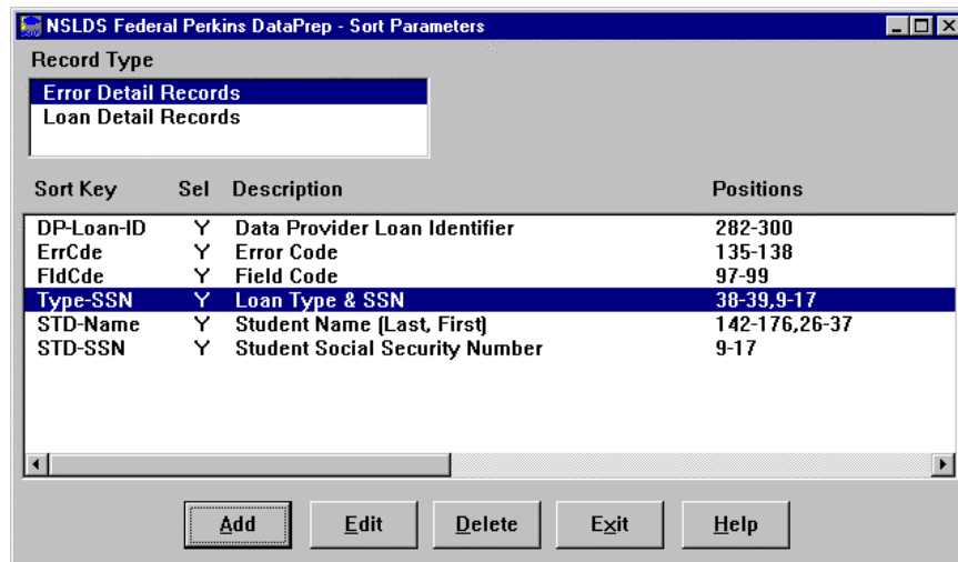
Figure 10-38: Sort Parameters Dialog Box
